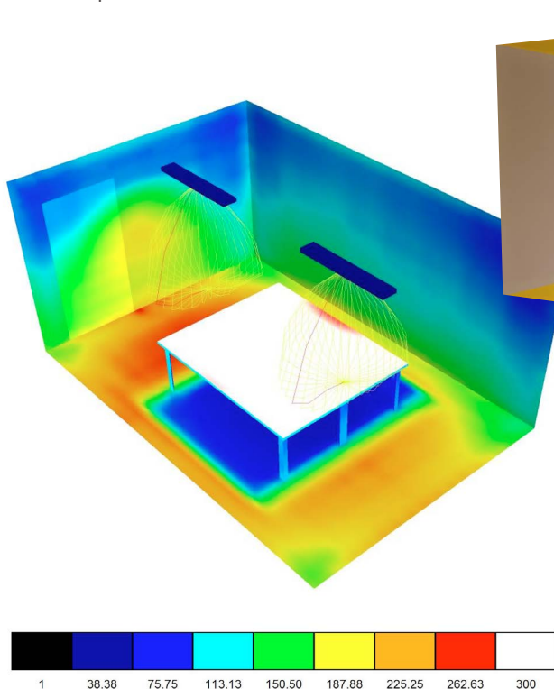
Simulation Dialux
